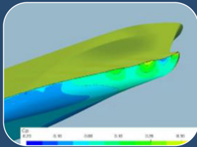
BOW OPTIMIZATION
